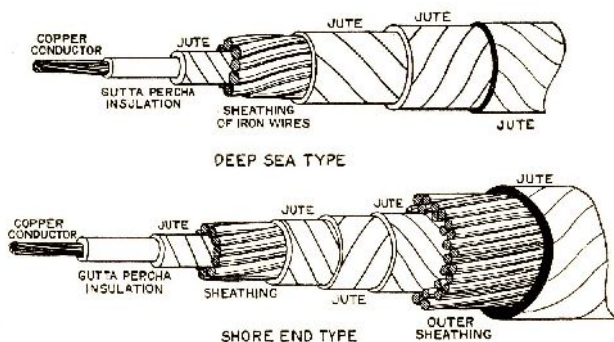
Fig. 116. Construction of Submarine Cable
